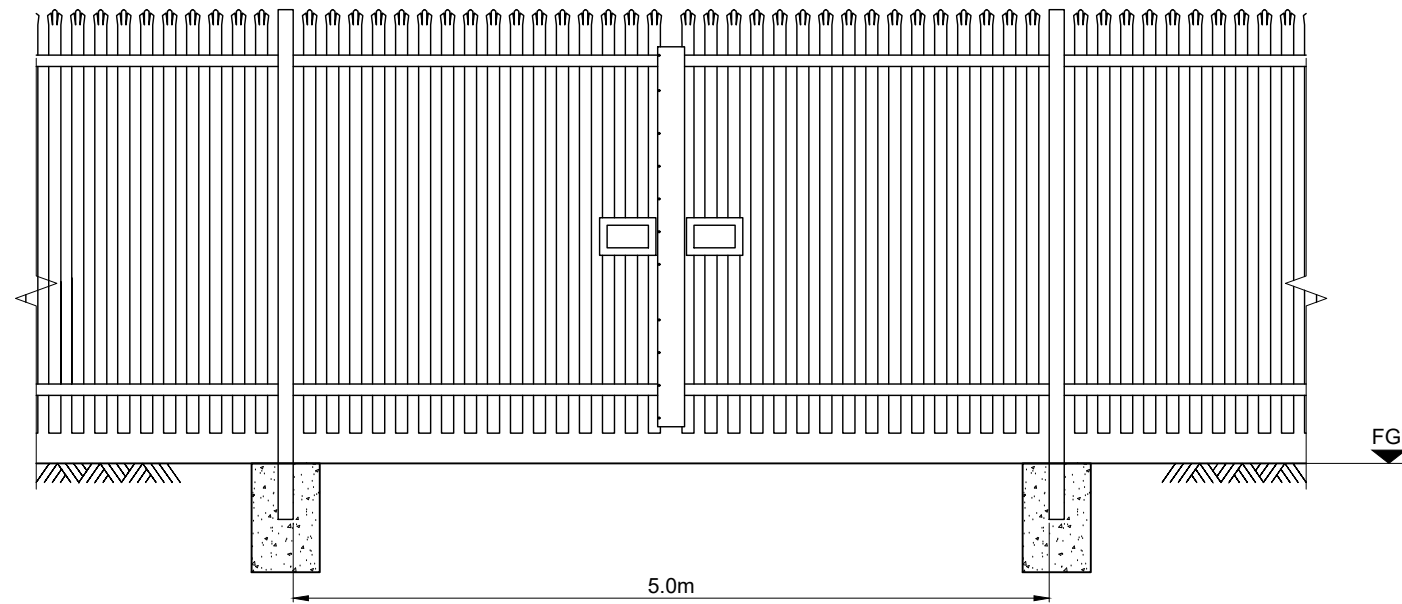
TYPICAL PALISADE FENCE ELEVATION (DOUBLE VEHICLE GATE)
