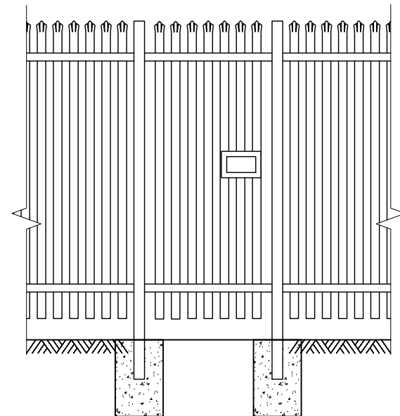
TYPICAL ELEVATION (PEDESTRIAN GATE)
